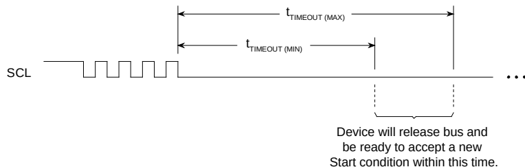
Figure 6-5. SMBus Timeout
